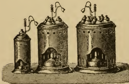
Fig. 50. KUNI'S APPARATUS FOR TESTING THE BAKING VALUE OF FLOUR.
